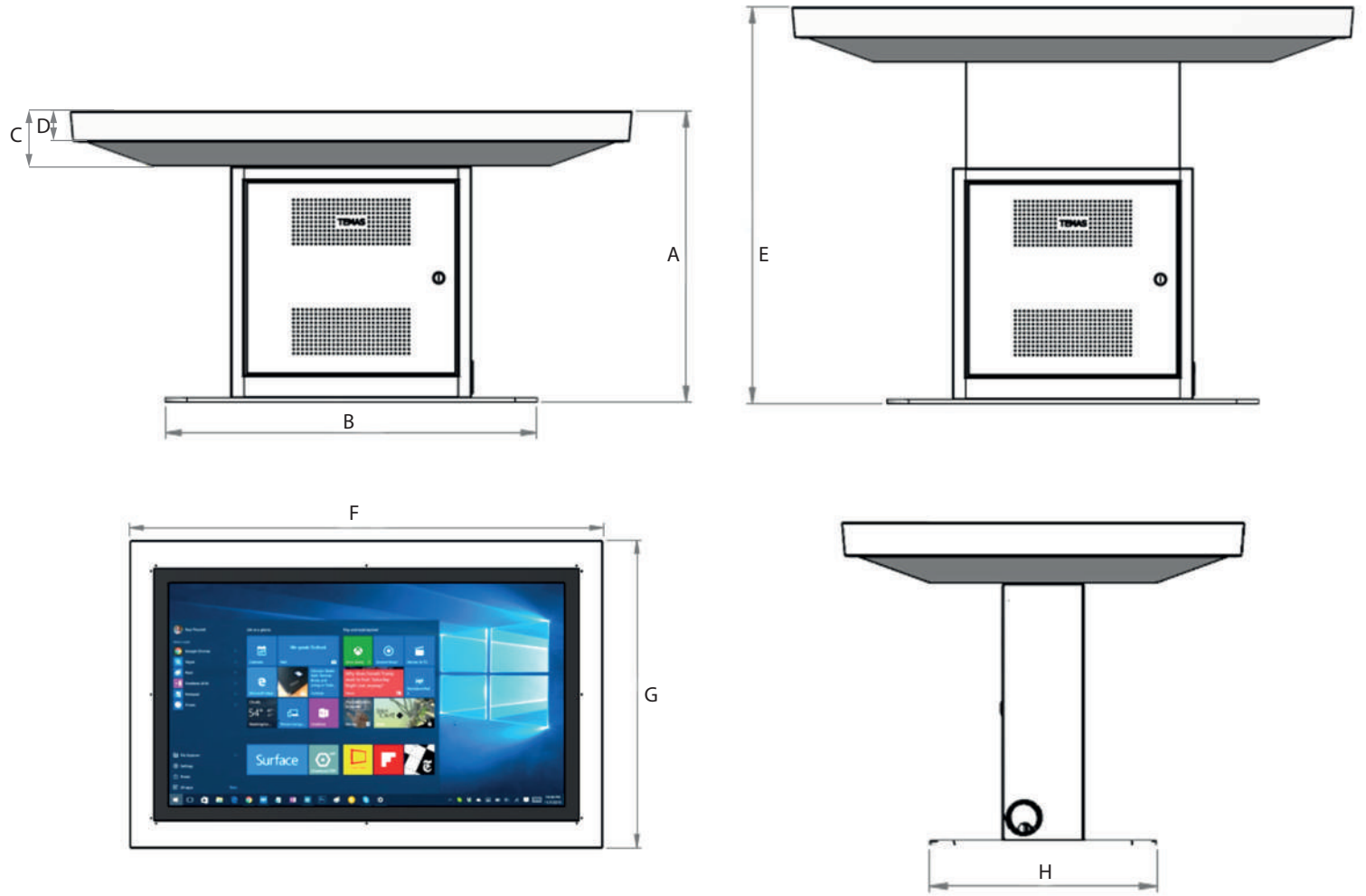
Dimension (mm)
